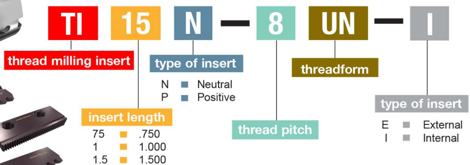
TC Series Thread Milling Insert Nomenclature Chart
