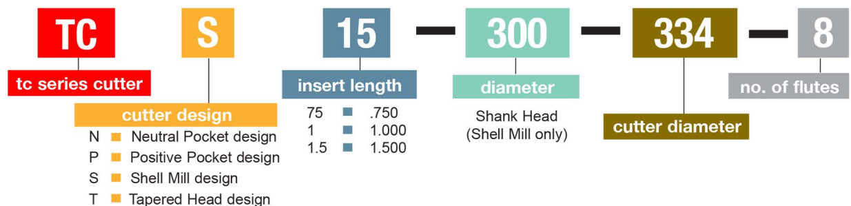
TC Series Thread Milling Cutter Nomenclature Chart
